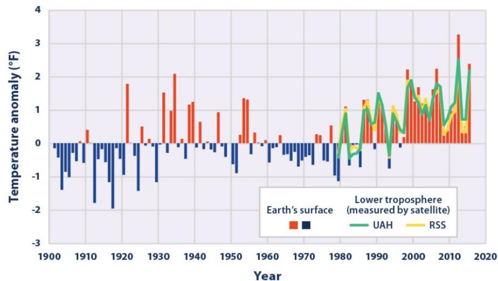
Figure 1. Temperatures in the Contiguous 48 States, 1901-2015
